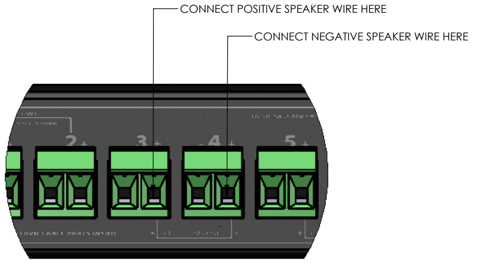
DETAIL B : CH 3/4 BTL OPERATION SCALE 1 : 1
