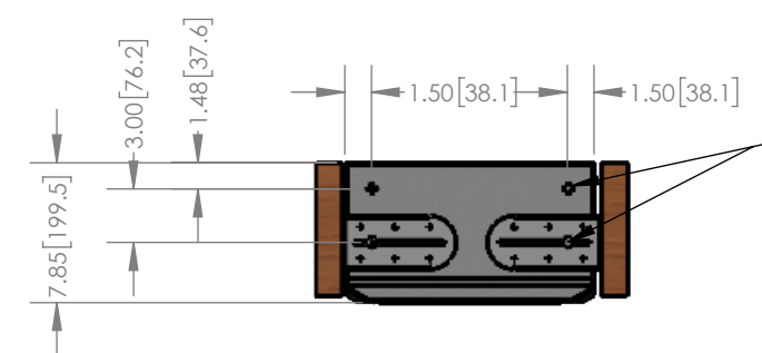
TOP VIEW (INSTALLED)
