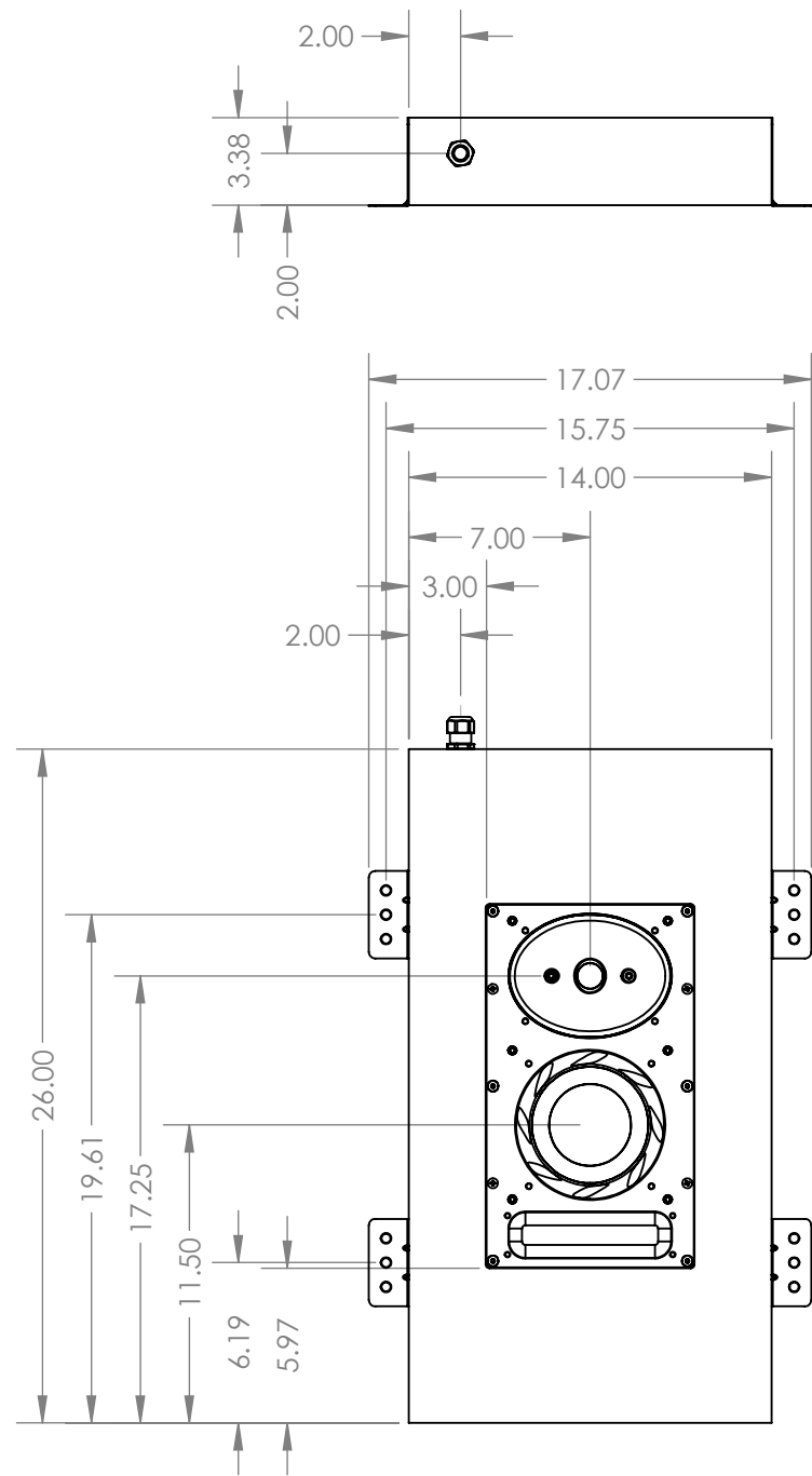
FRONT VIEW SPEAKER ASSEMBLY WITH ENCLOSURE
