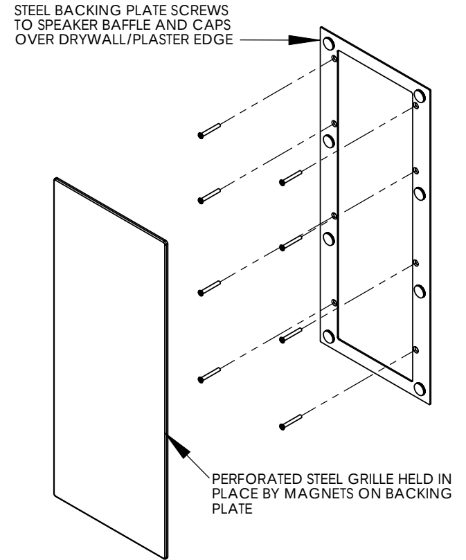
EXPLODED VIEW
